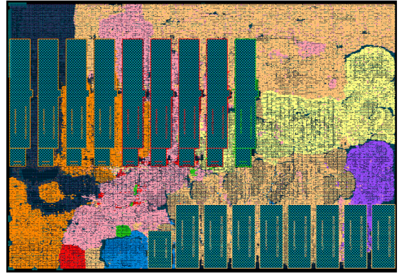
Figure 5: Data-parallel processor layout results
